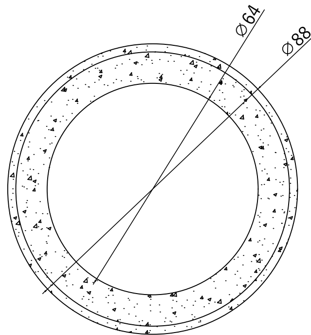
Vedere in plan Inel aducere in cota DN625 H100 G120
