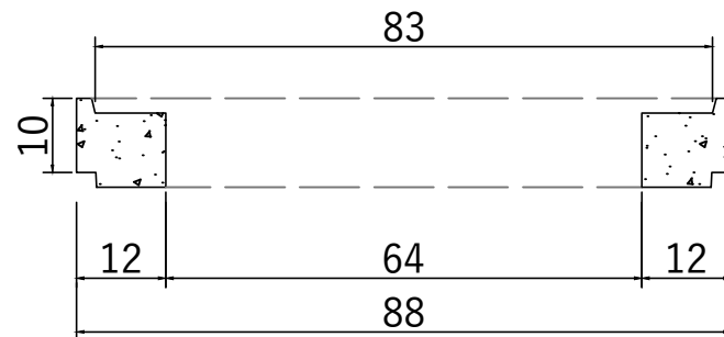
Sectiune Inel aducere in cota DN625 H100 G120
