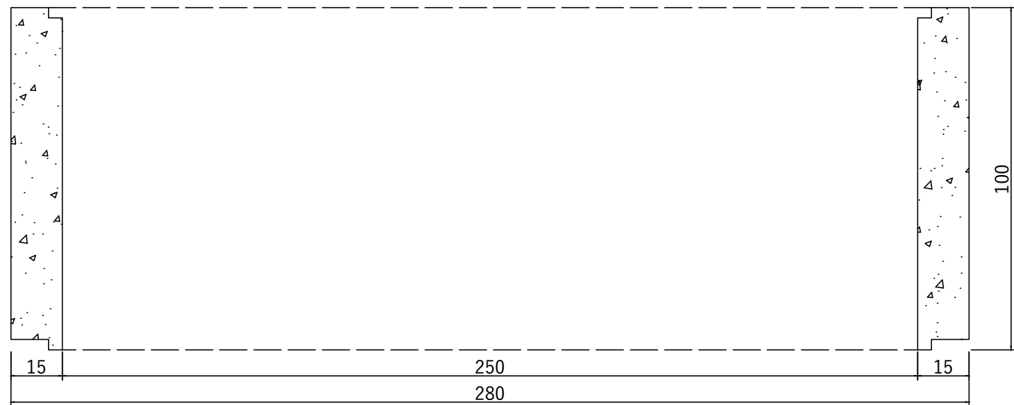
Sectiune Inel Bazin Circular DN2500 H1000 G150
