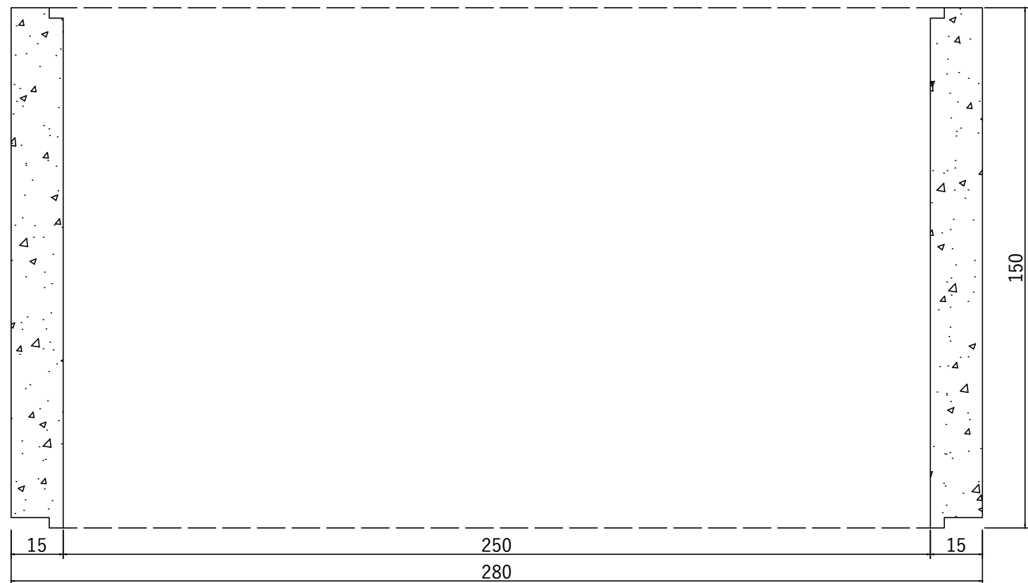
Sectiune Inel Bazin Circular DN2500 H1500 G150
