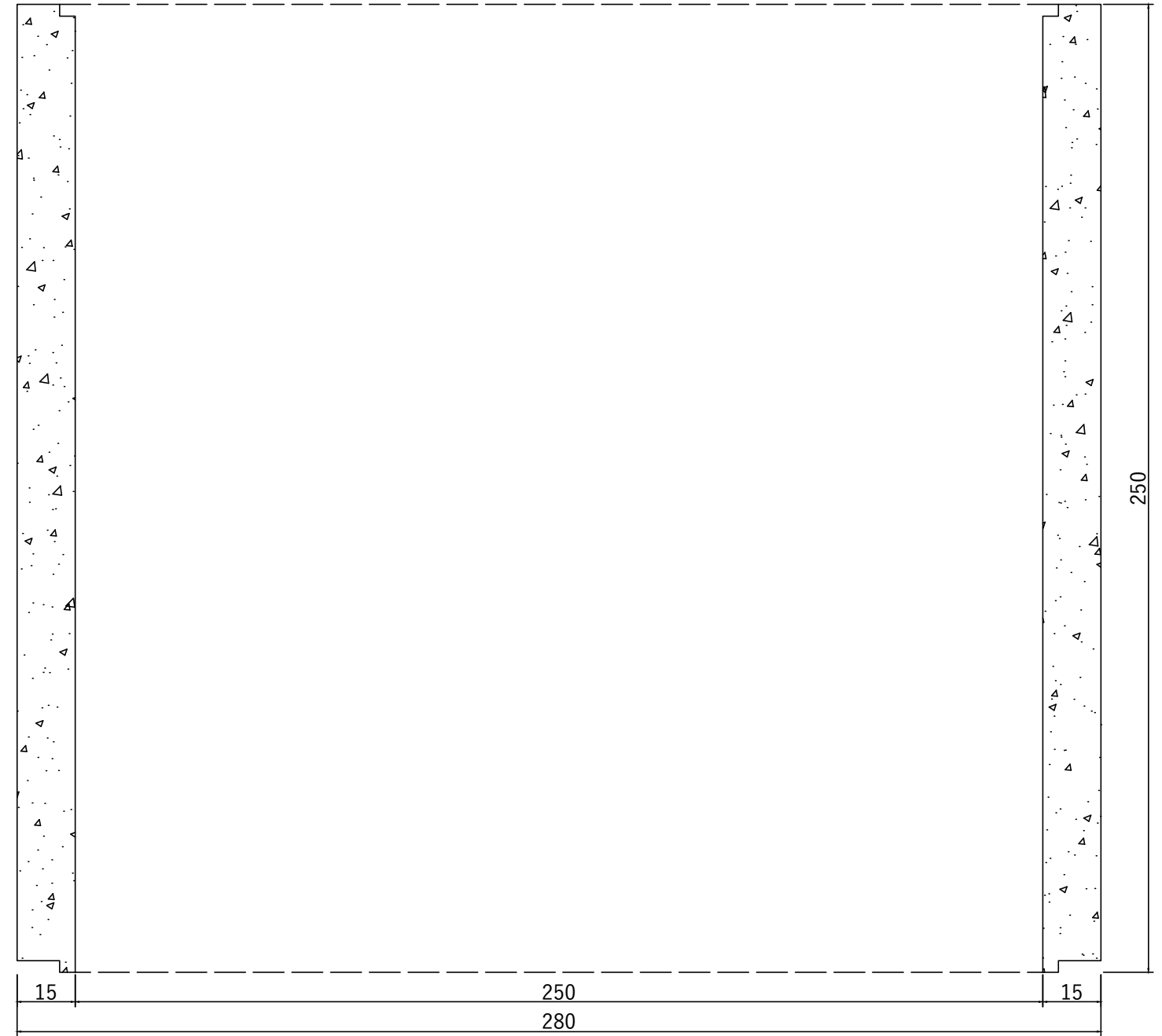
Sectiune Inel Bazin Circular DN2500 H2500 G150
