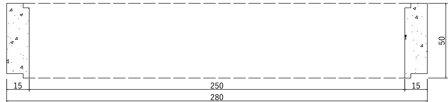
Sectiune Inel Bazin Circular DN2500 H500 G150
