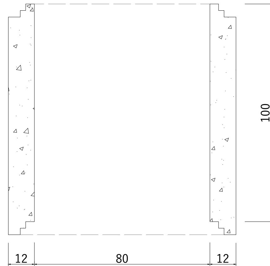
Sectiune Incel camin DN800 H1000 G120
