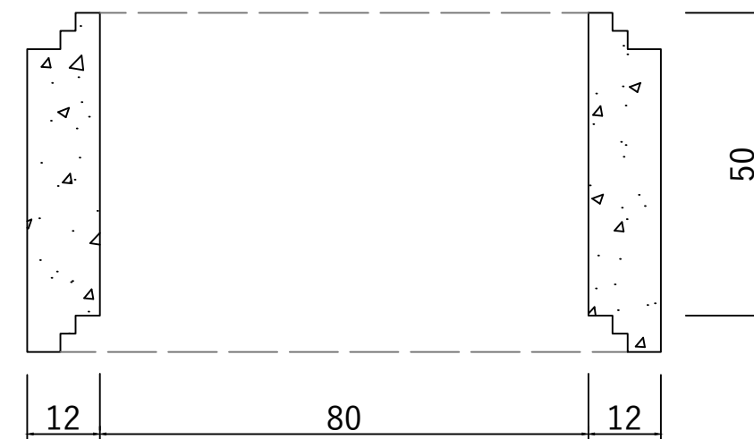
Sectiune Inel camin DN800 H500 G120
