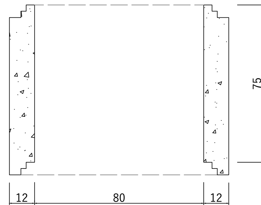
Sectiune Incel camin DN800 H750 G120
