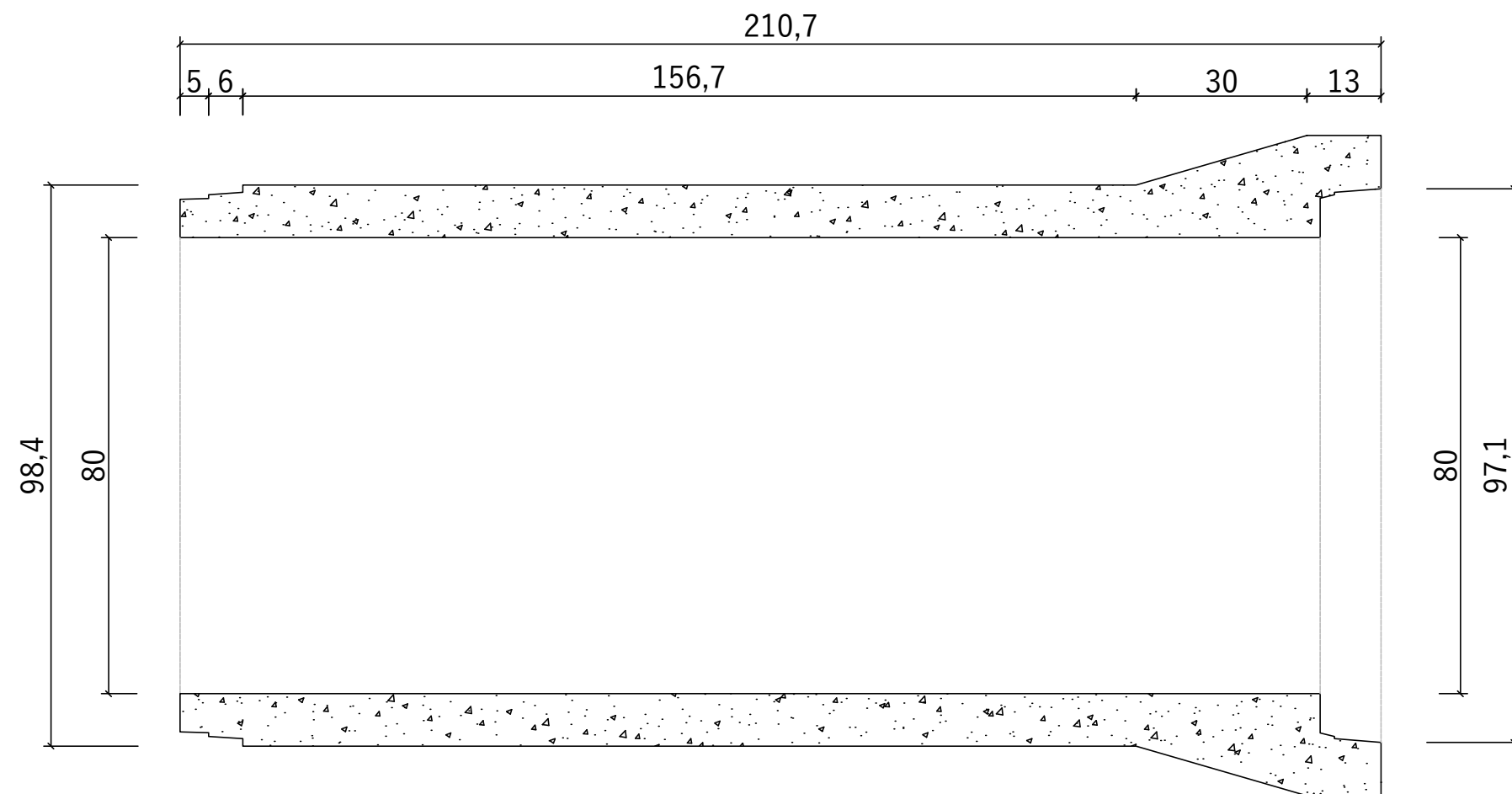
Sectione Tub beton Ø 800mm
